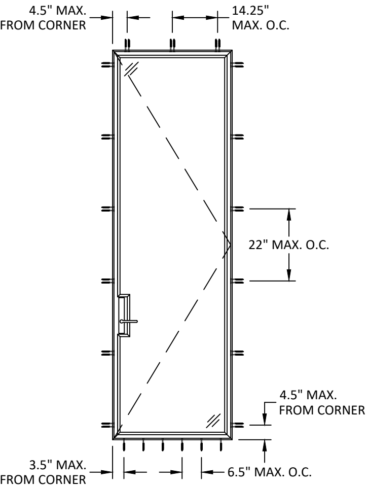
ANCHOR LAYOUT SINGLE DOOR
