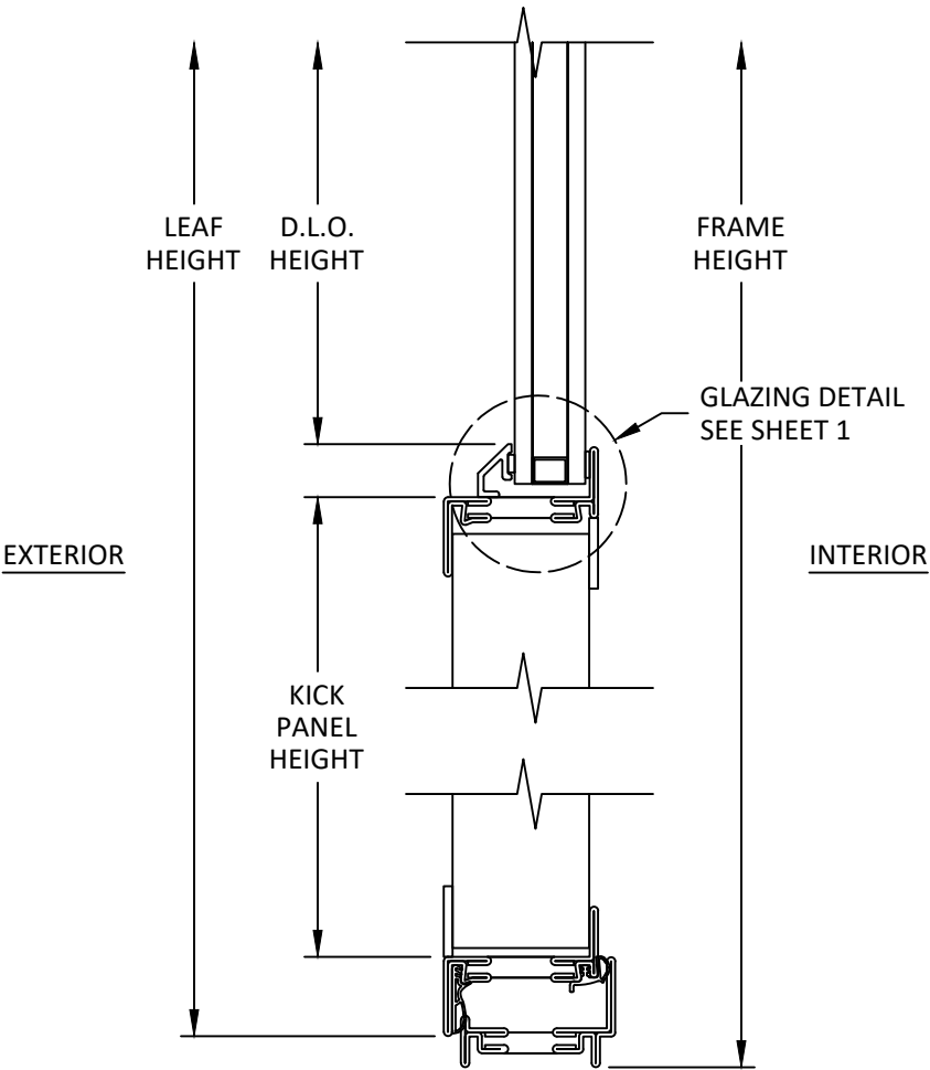
C 5 VERTICAL SECTION SILL WITH KICK PANEL
