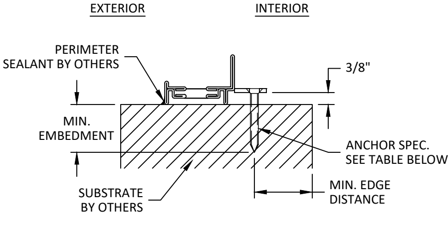
H 7 INSTALLATION DETAILS SILL SHOWN
