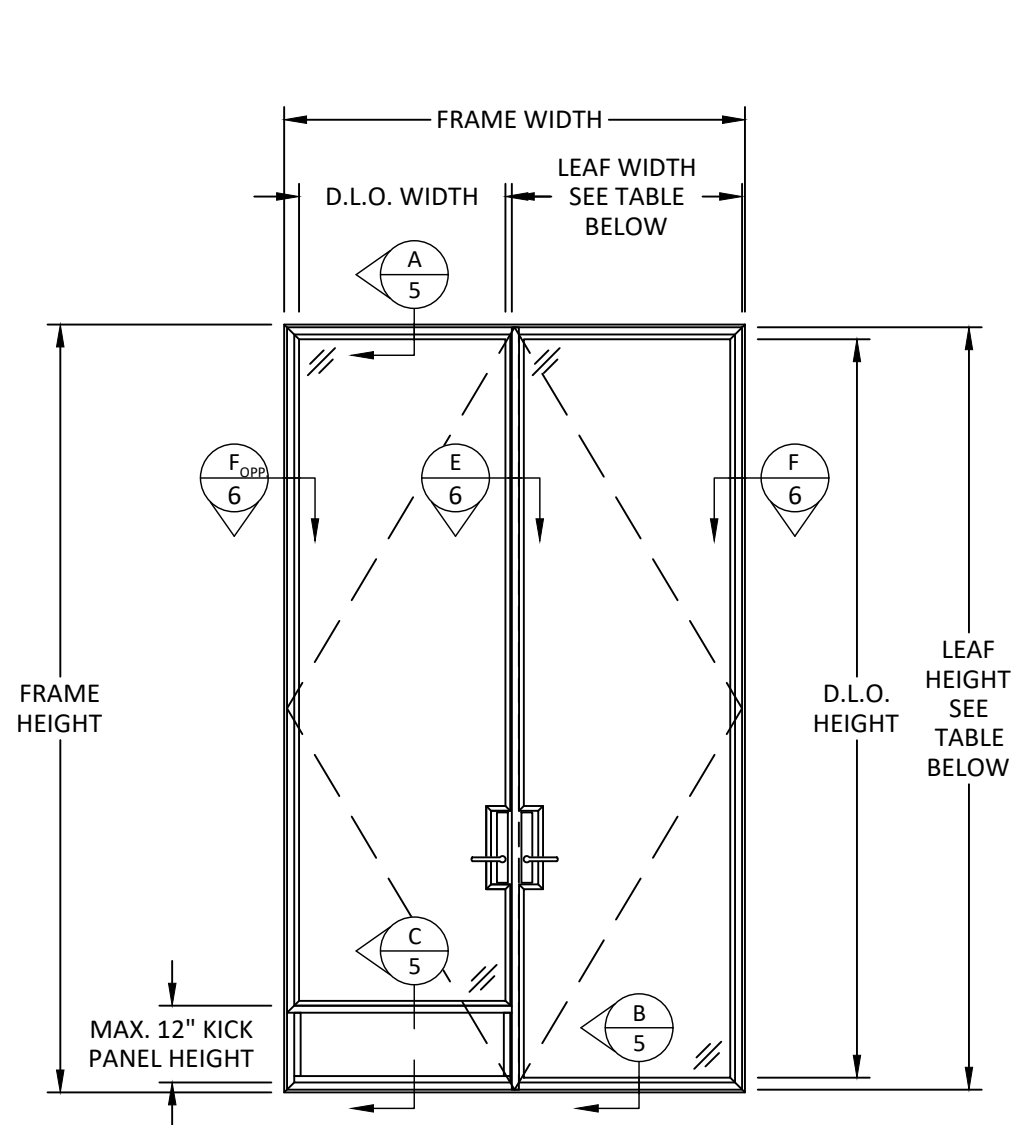
TYPICAL ELEVATION FRENCH DOOR
