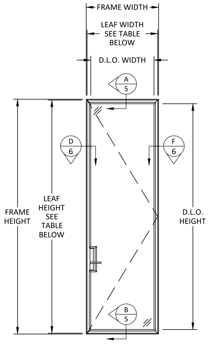
TYPICAL ELEVATION SINGLE DOOR
