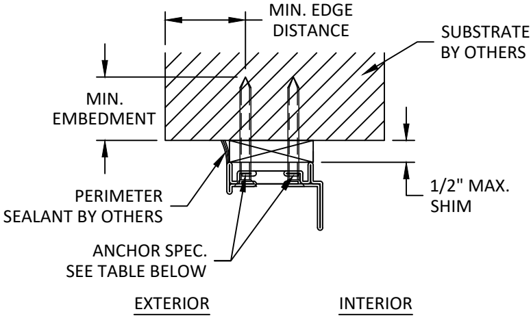
G 7 INSTALLATION DETAILS HEAD SHOWN JAMB SIMILAR
